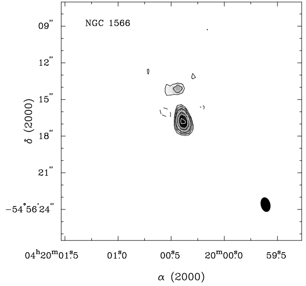
Fig. 7. NGC 1566. Contours: -0.9, -0.6, 0.6, 0.9, 1.4, 2.2, 3.4, 5.3 mJy beam -1
